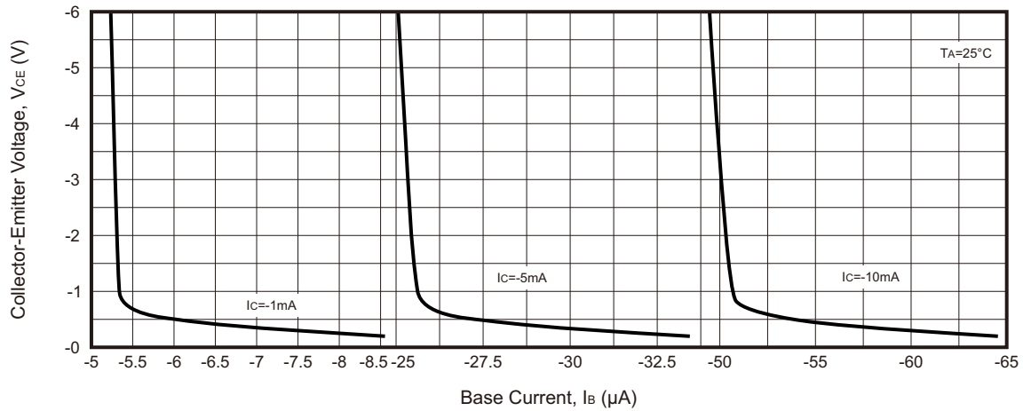
Fig.1 - Static Characteristic
